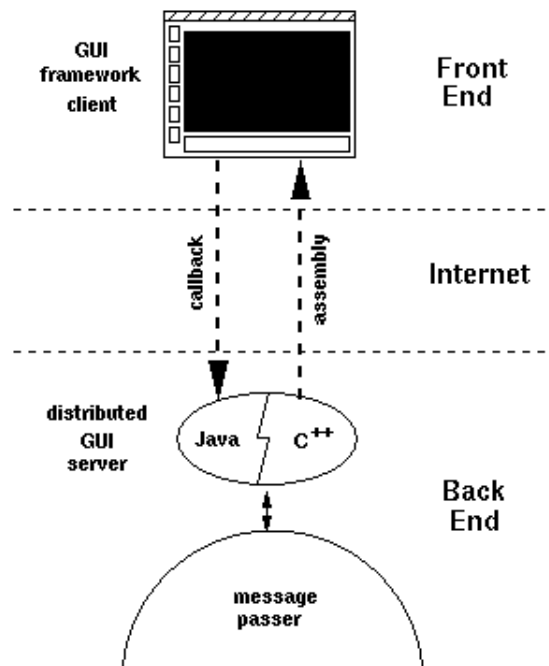
Figure 3: Communication within the distributed GUI framework architecture.
